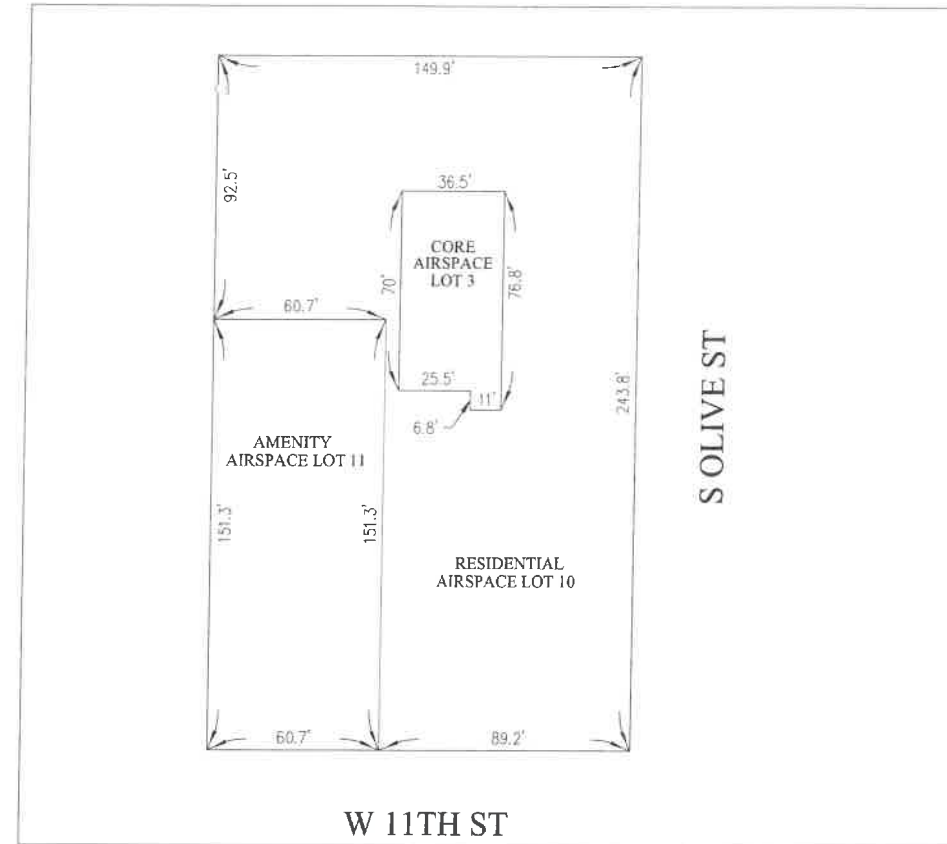
LEVEL L11 AIRSPACE LOTS 3,10,11
